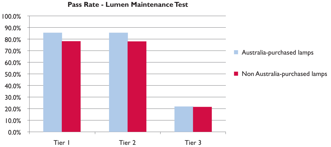
Figure 17. Lumen Maintenance Test Pass Rate for ALC Tiers 1, 2 and 3
