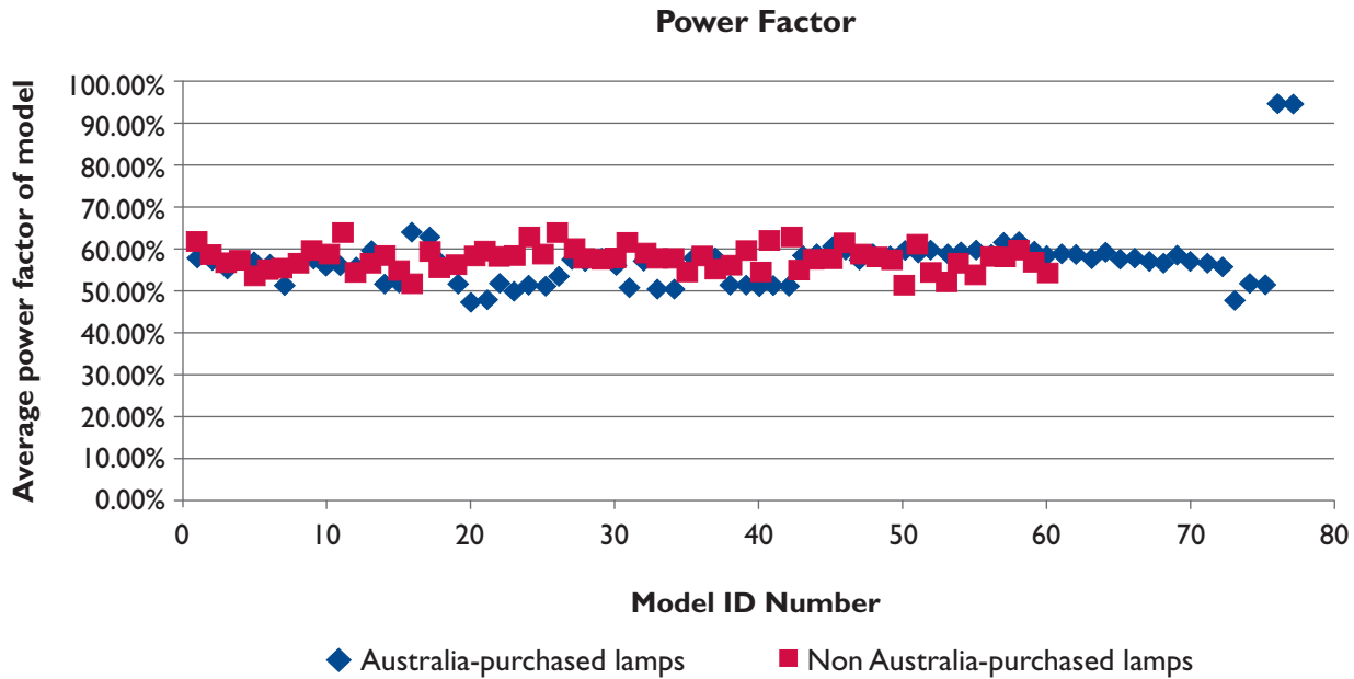
Figure 18. Average Power Factor Results for All 137 Models Tested
